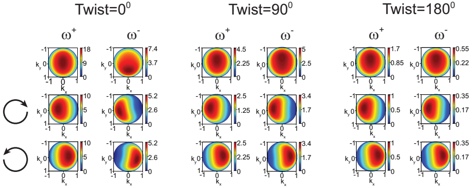
Figure 7.2: Radiation patterns of split ring stereodimers with 0^\circ , 90^\circ and 180^\circ twist angle. The radiation patterns in the second and third row are polarization analyzed with circular polarizer of handedness that is depicted by the black arrows on the left hand side.
