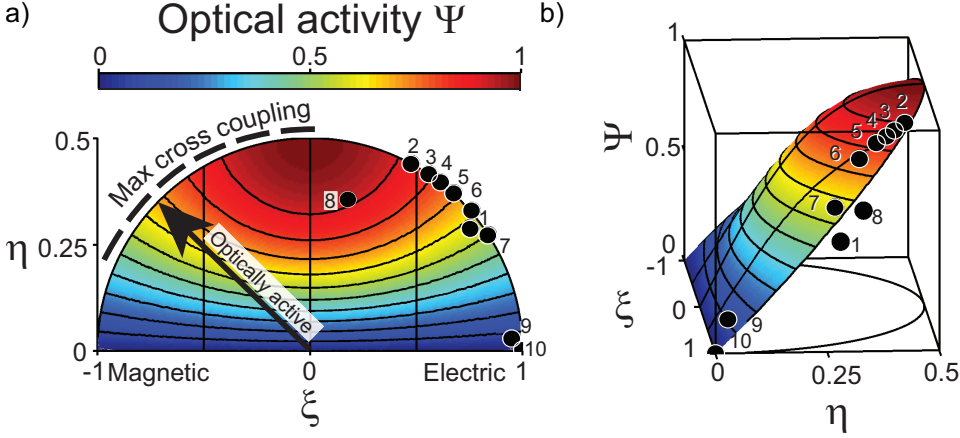
Figure 5.4: Master diagrams summarizing optical activity and bi-anisotropy mapped as a function of \xi = (\alpha_E - \alpha_H)/((\alpha_E + \alpha_H)) and \eta = (\alpha_C)/((\alpha_E + \alpha_H)) . All structures we tested (data-points, numbered as in Fig. 5.1(b)) are close to the locus of maximum cross coupling (ellipse), except (8). The color scale shows optical activity contrast \Psi , in the dipole approximation (color scale) and for tested structures (dots). Panel (b) is a 3D representation of (a).
