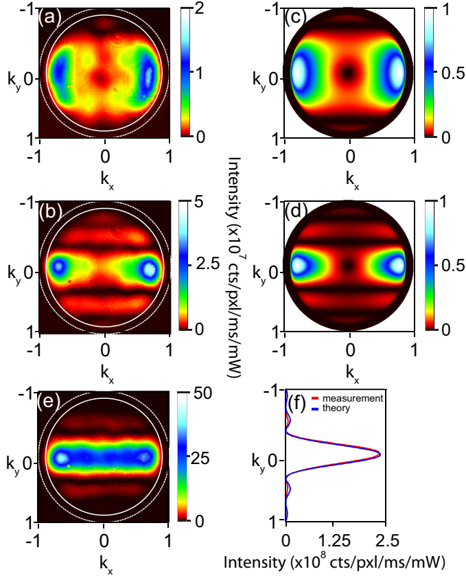
Figure 6.4: (a) Fourier space image of a 1 \mu\text{m} long, 50 nm wide and 30 nm thick Au nanowire excited by p-polarized incident light. (b) Fourier space image of a 2 \mu\text{m} long, 50 nm wide and 30 nm thick Au nanowire excited by a p-polarized incident light. (c) and (d) are calculated radiation patterns of 2 \mu\text{m} and 1 \mu\text{m} long Au nanowires multiplied by the transmission function, respectively. (e) Fourier space image of a 2 \mu\text{m} long, 50 nm wide and 30 nm thick Au nanobar excited with s-polarized incident light. The nanobars are excited at 725 nm and 200 \mu\text{W} . The total exposure time is 1 s in (a), 100 ms in (b), and 10 ms in (e). (f) An average cross-cut of (e) along k_y (red curve) agrees well with the calculated \text{sinc}^2 behavior (blue line).
