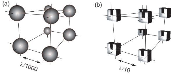
Figure 1.2: (a) A schematic of a simple cubic crystal consisting of atoms (grey circles). (b) A schematic of the same cubic crystal with split rings as atoms.
