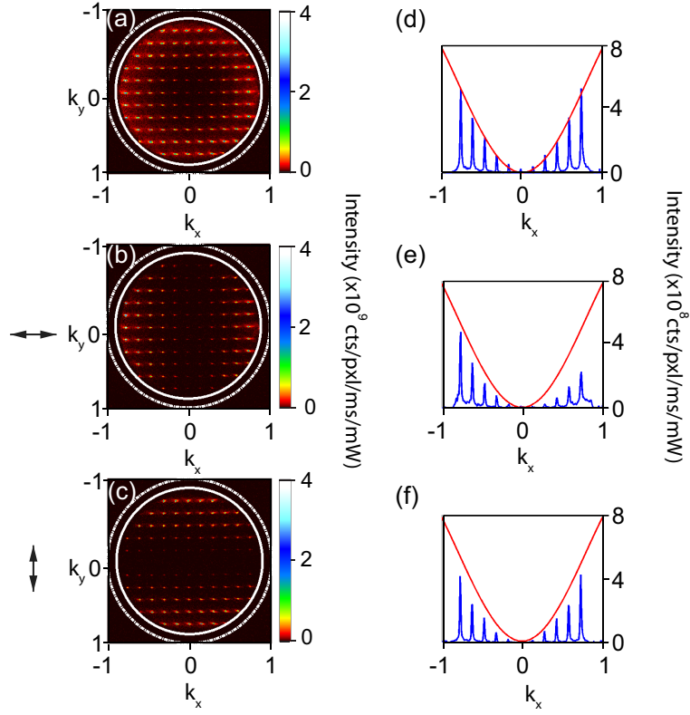
Figure 6.3: (a) Fourier space image of a periodic square array of 200 nm long, 50 nm wide and 30 nm thick Au nanobars with 4 μm lattice spacing excited with p-polarized incident light at 600 nm with 20 μW. The total exposure time is 10 ms. (b), (c) Radiation patterns under the same illumination conditions as in (a) and polarization analyzed across (b) and along (c) the nanobar length, as denoted by the black arrows. (d), (e), (f) Fitted sin 2 (red line) to cross sections along the central column ((a), (c)) and row ((b)) of grating orders in our measurements in (a), (b) and (c), respectively, with a scaling factor of 11 \times 10^8 and an offset of 3 \times 10^6 counts per pixel, per mW incident power and per ms exposure time.
